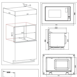
2 Microwave oven cabinet
